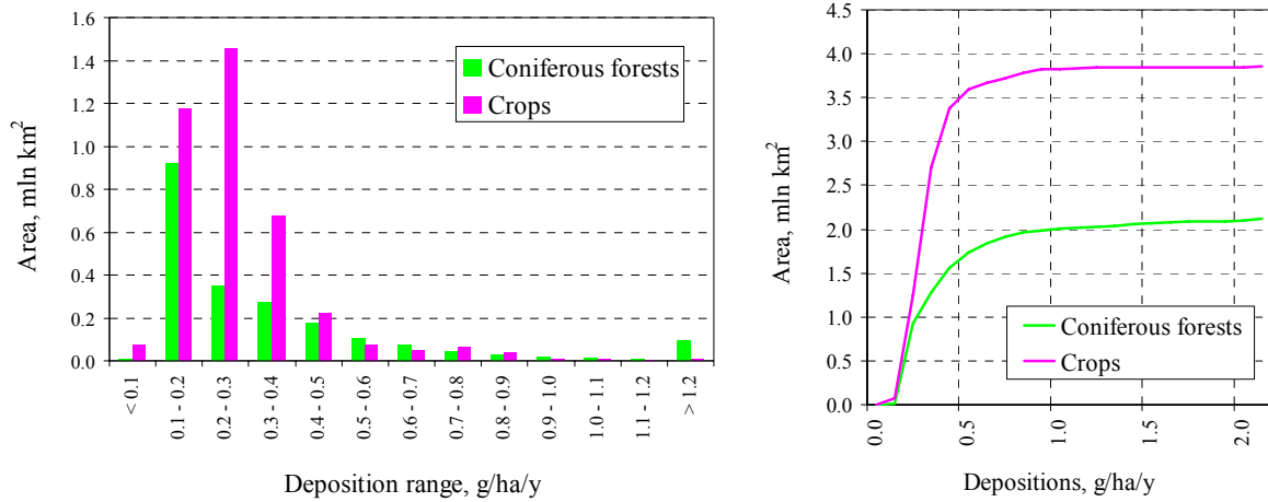
Figure 4-15. Area distribution function (left) and cumulative distribution function (right) of total deposition flux of cadmium in 2000.
