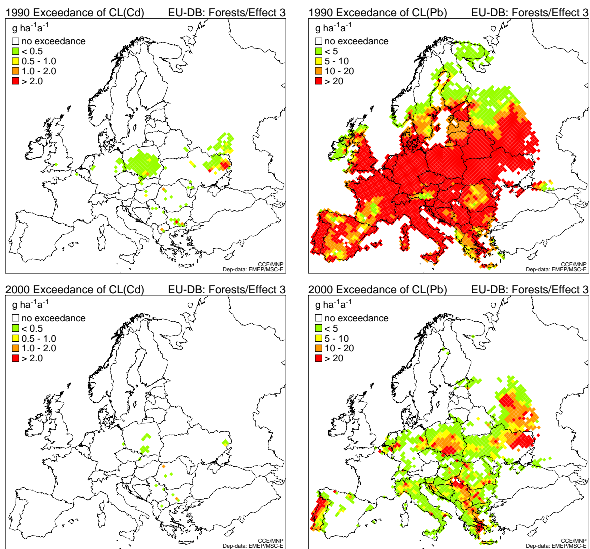
Figure 3-2. Exceedances of the EU-DB critical loads of cadmium (left) and lead (right) for ecotoxicological effects in forests on the EMEP50 grid in the year 1990 (top) and 2000 (bottom).
