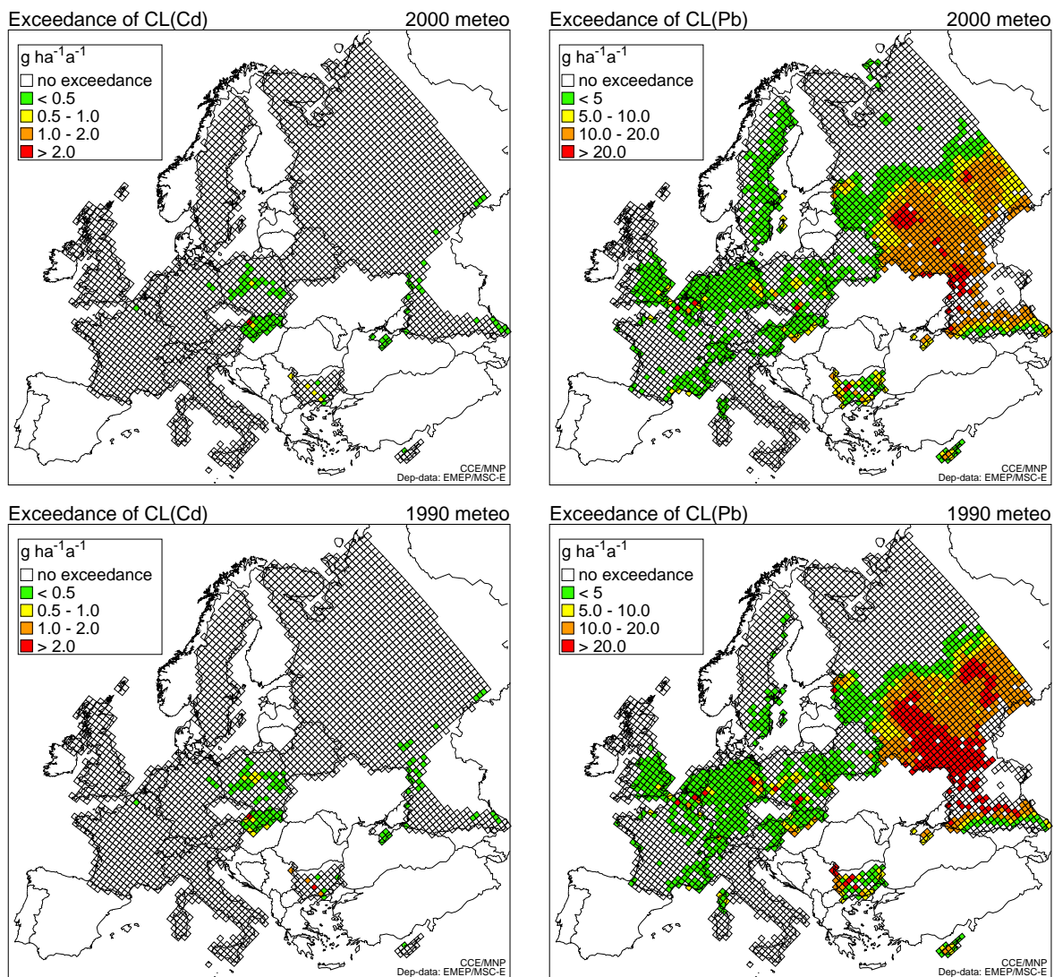
Figure 5-7. Exceedance of CL(Cd) (left) and CL(Pb) (right) with the actual depositions in 2000 (top) and the 2000 depositions calculated with 1990 meteorological data (bottom).
