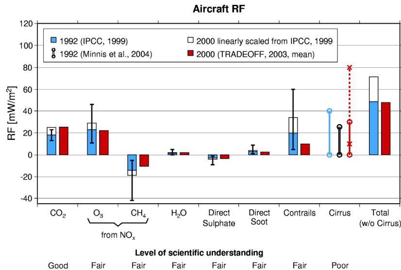
Figure 1 RF [ mW/m^2 ] from aviation for 1992 and 2000, based on IPCC (1999) and TRADEOFF results.
