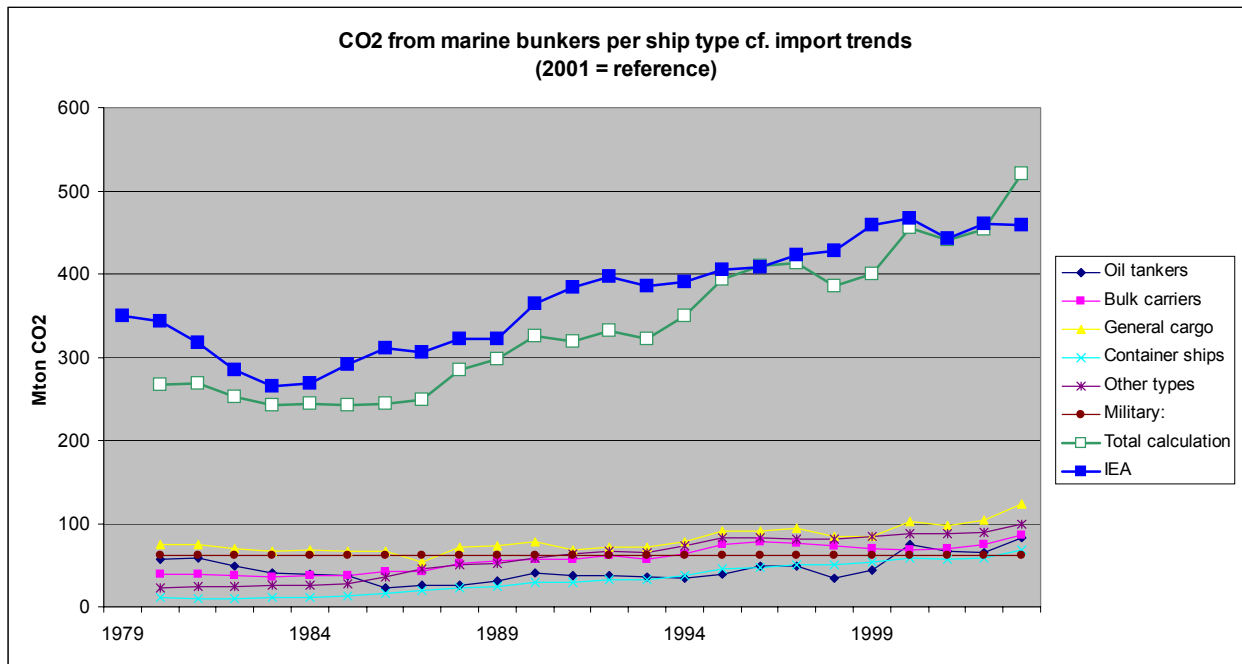
Figure A.5. Comparison of CO 2 emissions reported by IEA (2005) and calculated from import values per ship type (UNCTAD, 2006), assuming constant specific fuel consumption (GJ/US$, calculated for 2001).
