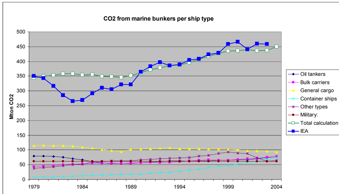
Figure A.4. Comparison of CO 2 emissions reported by IEA (2005) and calculated from DWT volume per ship type
