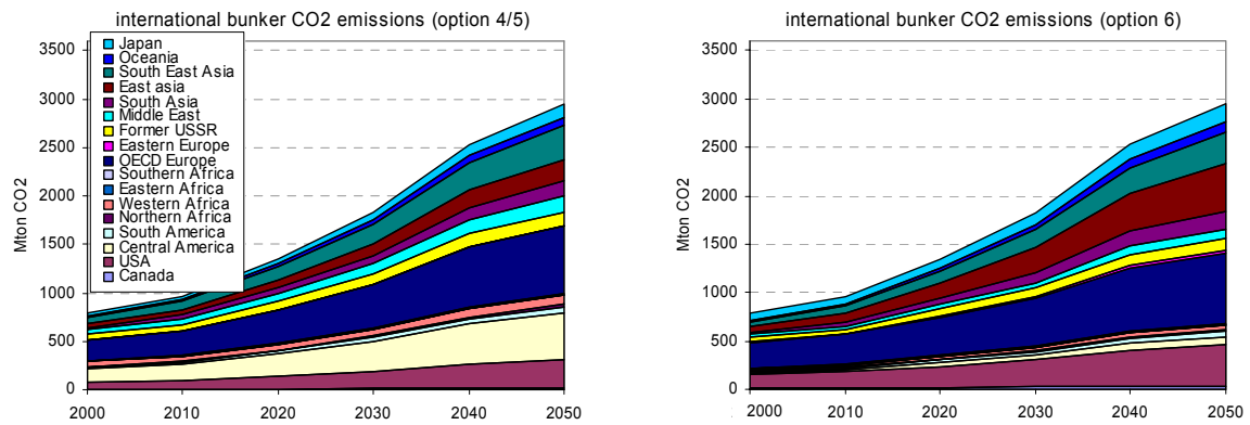
Figure 9 The international bunker emissions for the IPCC SRES baseline B2 scenario as constructed for this study for the option 4/5 (i.e. option 4 for marine (flag state) and option 5 for aviation (destination aircraft)) (left) and option 6 marine and aviation (destination passenger/cargo) (right). Source: Den Elzen, 2006, Den Elzen 2007.
