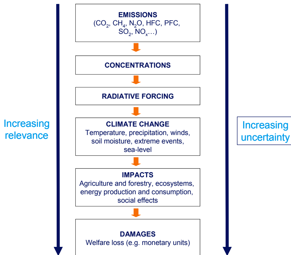
Figure 3 Overview of chain between emissions and 'damage'. Source: Fuglestvedt, 2003 and IPCC, 2001, Chapter 7.
