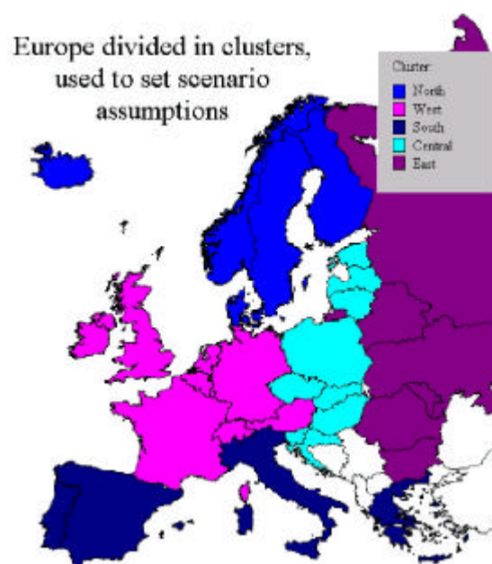
Figure 29. Clustering of European countries (Source: Huisman and Imhoff, 1999).
