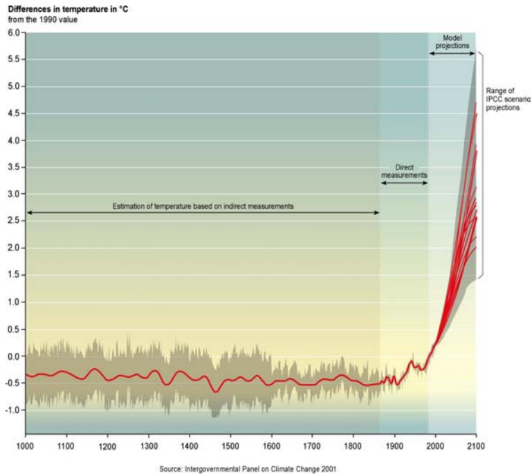
Figure 3.20. Historic and Projected Variations of the Earth's Surface Temperature
