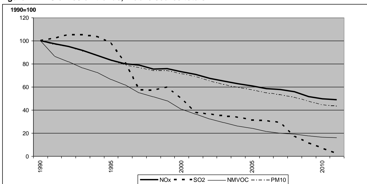
Figure B. NEC emission trends, mobile source totals
