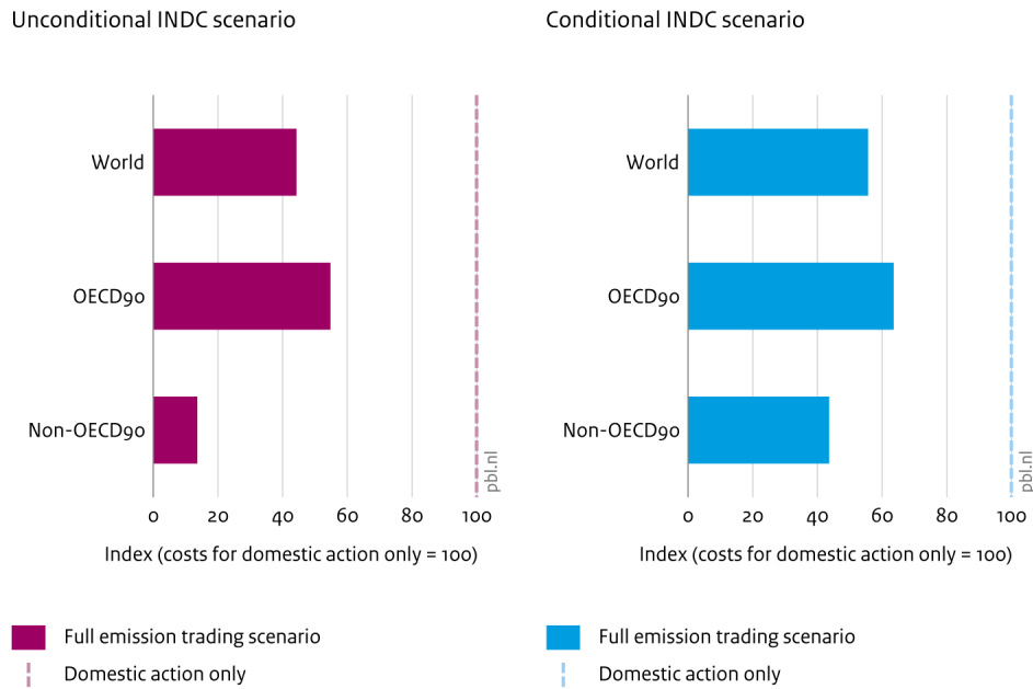
Figure 3 Impact of full emission trading on abatement costs for INDCs under the SSP2 baseline, 2030
