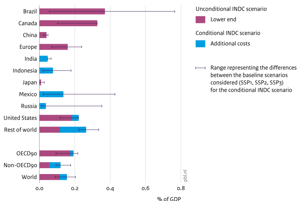
Figure 2 Abatement costs for INDCs under SSP2 baseline, 2030
