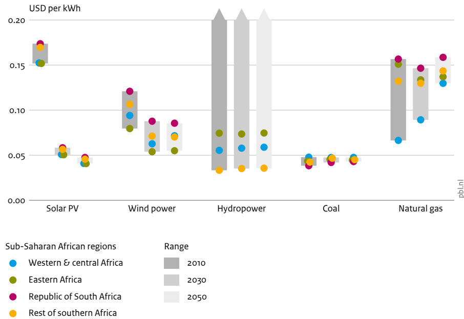
Figure 3.6 Levelised cost of electricity (LCOE) for central grid, per technology, under SSP2 baseline scenario
