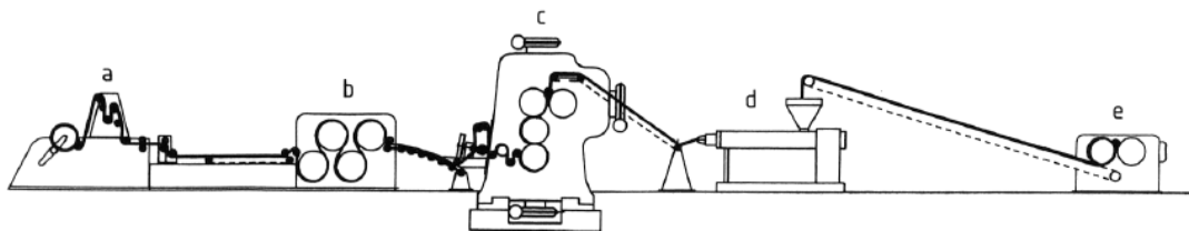
Figure 13: Calendaring line; a) Cutter; b) Cooling rolls; c) Four-roll calender; d) Extruder; e) Mixing roll mill (Ullman, 2016).
